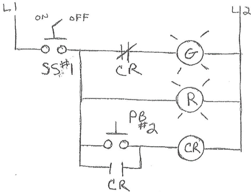
ALARM SILENCE CIRCUIT
